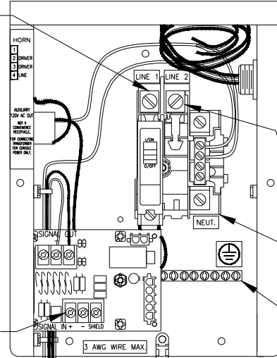
LOAD CENTER WITH COVER REMOVED
