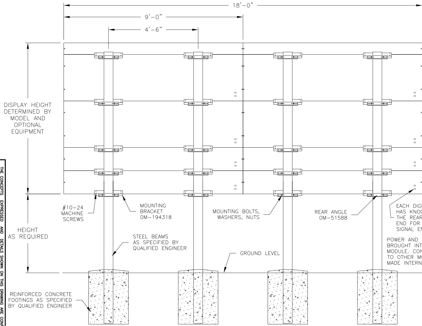
REAR VIEW TYPICAL HORIZONTAL DISPLAY
