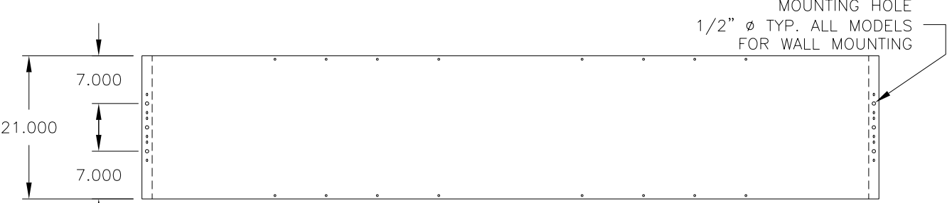
REAR VIEW 21" AD PANEL
