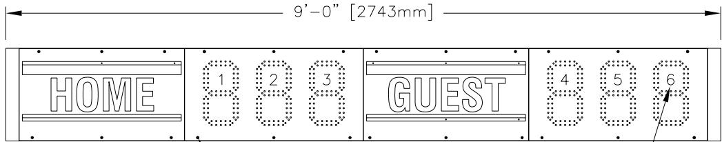
FRONT VIEW
