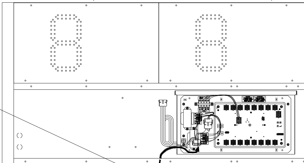
2-LINE MODULE (SHOWN WITH THE LOWER LEFT PANELS REMOVED)
