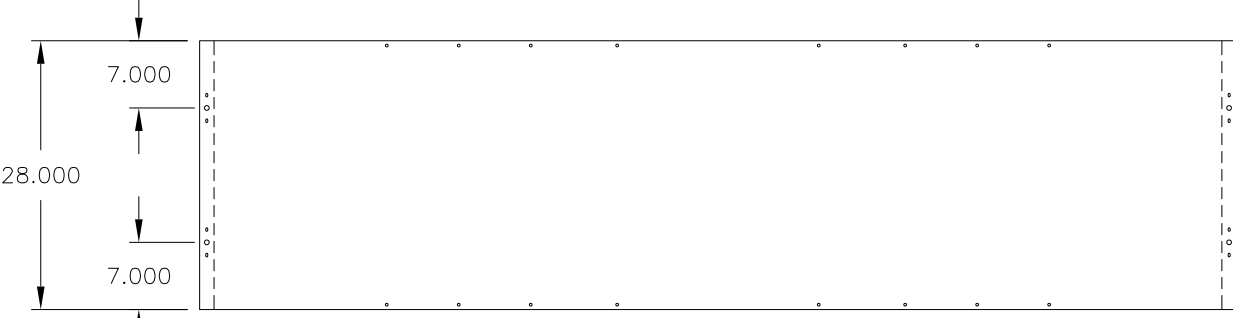
REAR VIEW 28" AD PANEL
